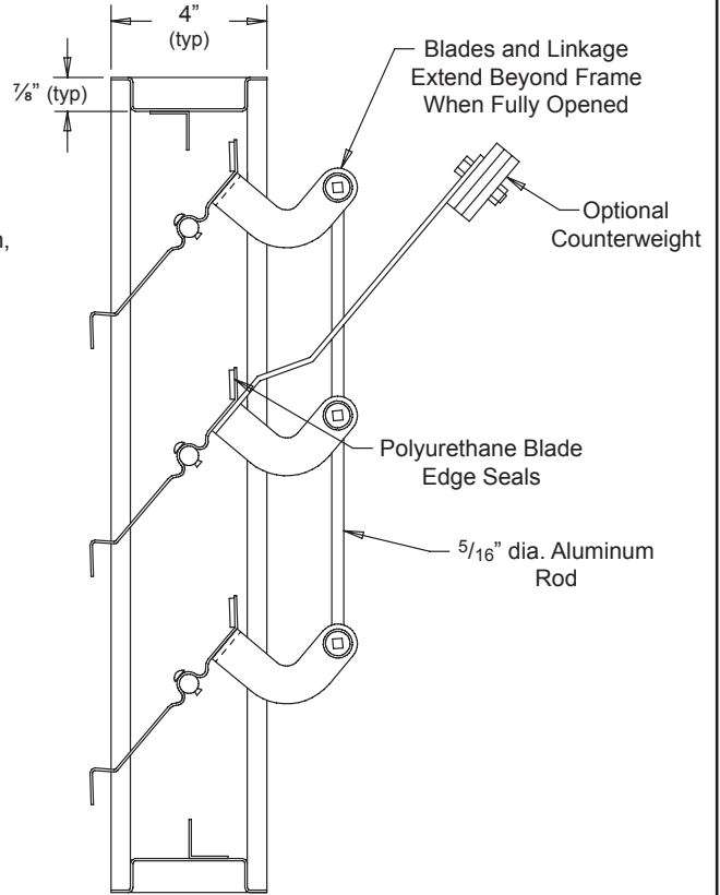
Section View
