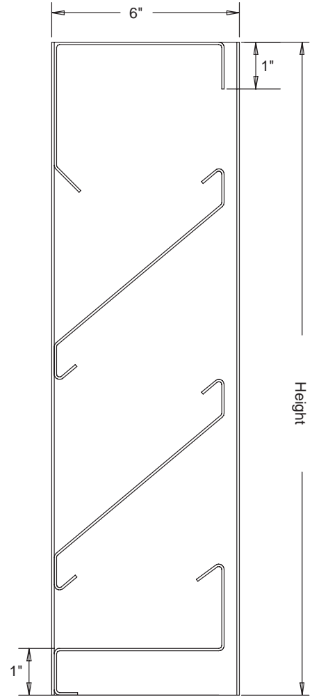
Section View
